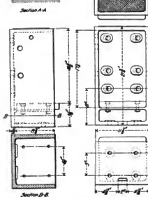
Figs. 3762-3767. Rear Upper Step.
